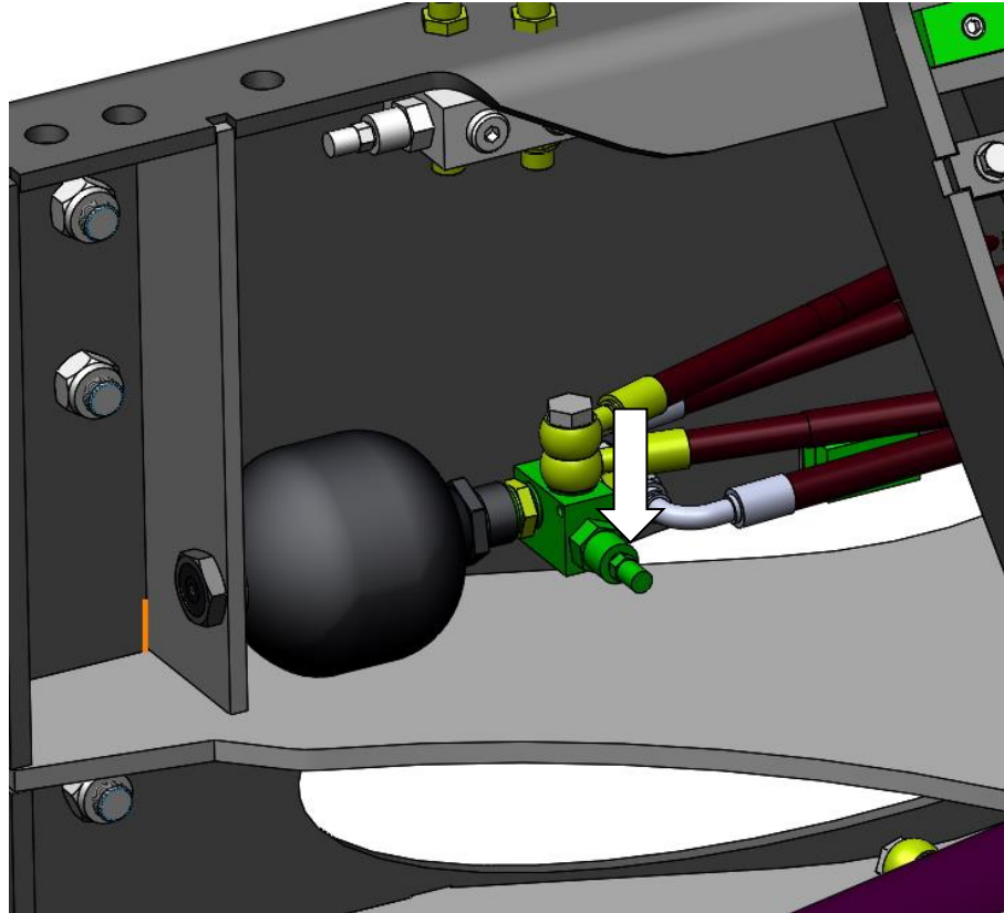
Picture 5. Pressure adjustment of the hydraulic suspension
