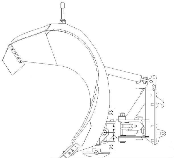
Picture 2. Floating bar in the mid position
