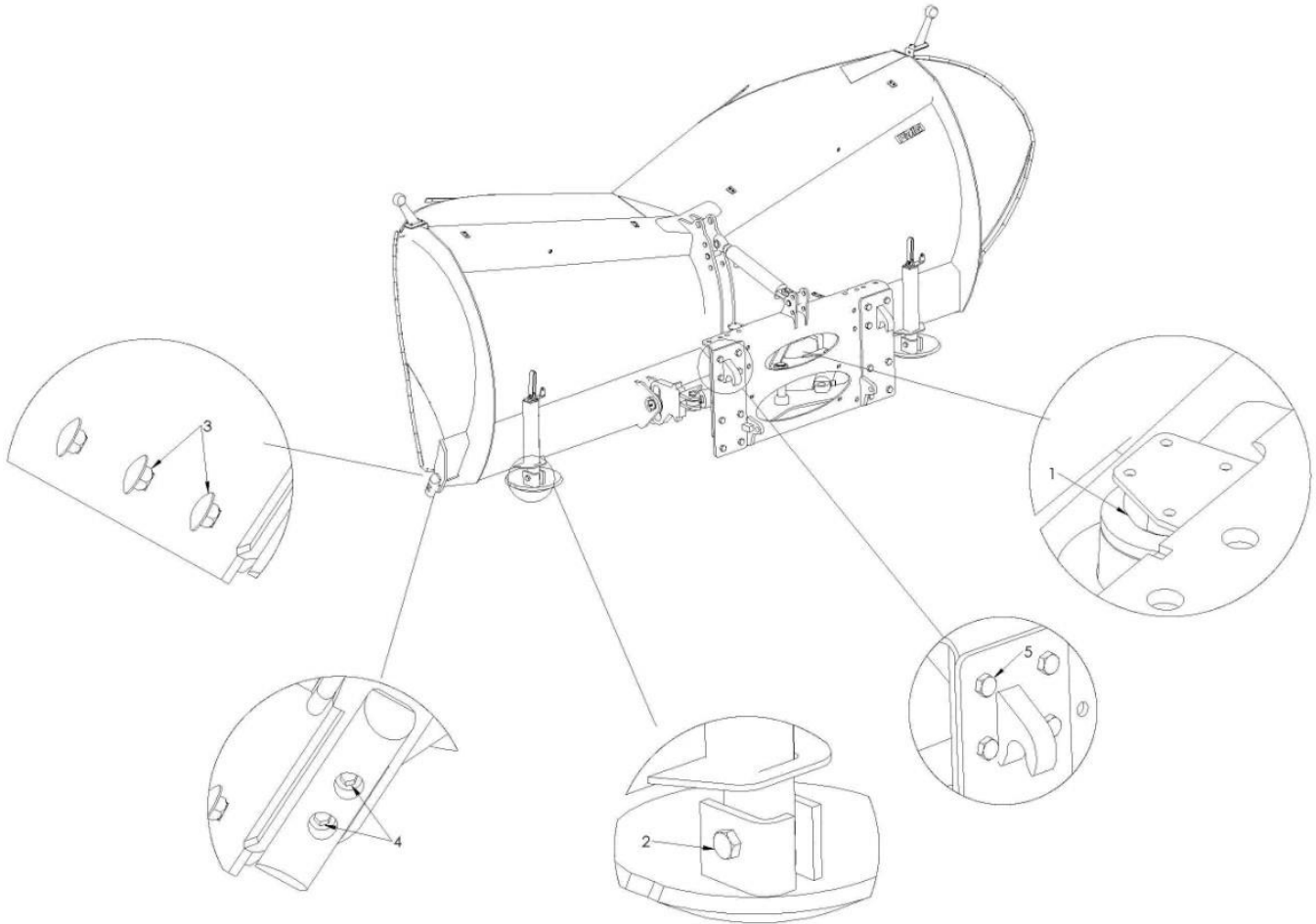
Picture 11. Screws to be tighten
