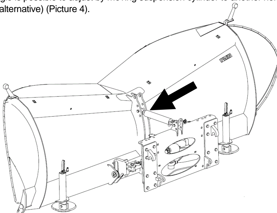
Picture 4. 3 holes for the hydraulic suspension cylinder
